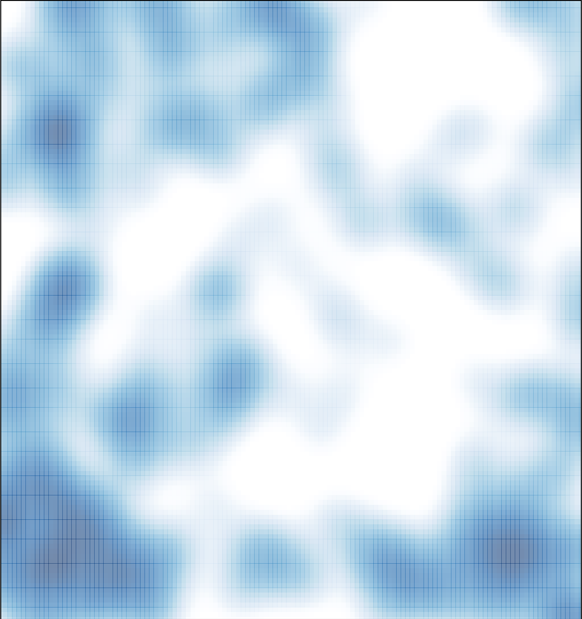
# features = 253 , max = 3
